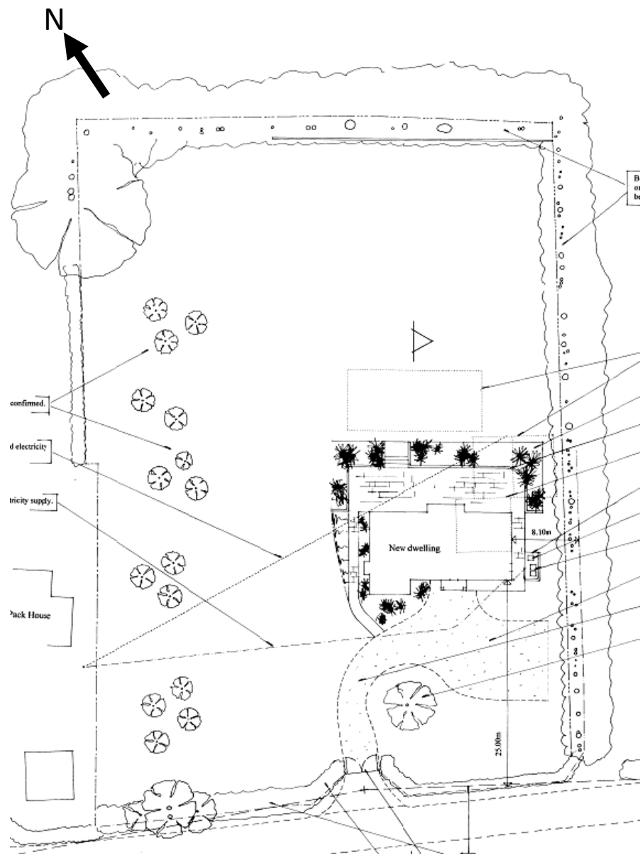
PROPOSED SITE PLAN WITH VIEWS FROM WITHIN SITE.
